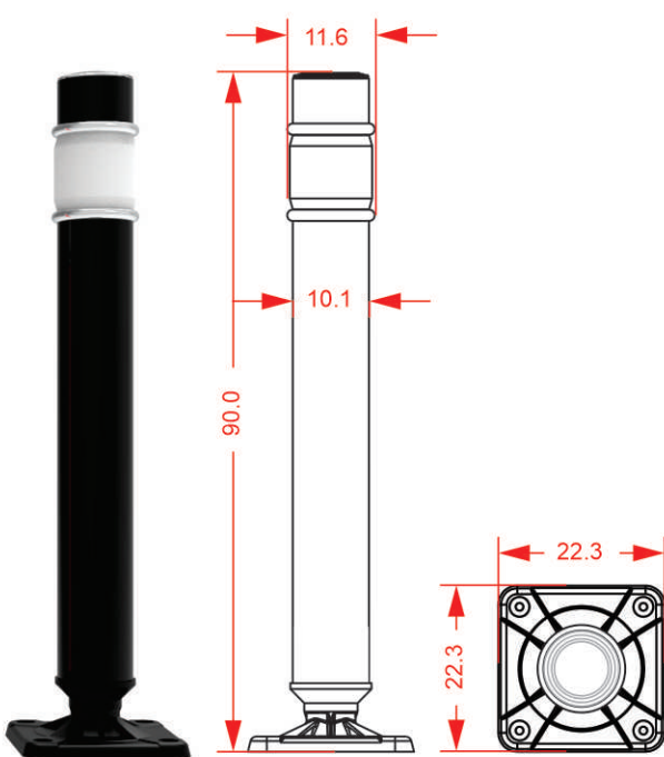
BOLARDO ABATIBLE
