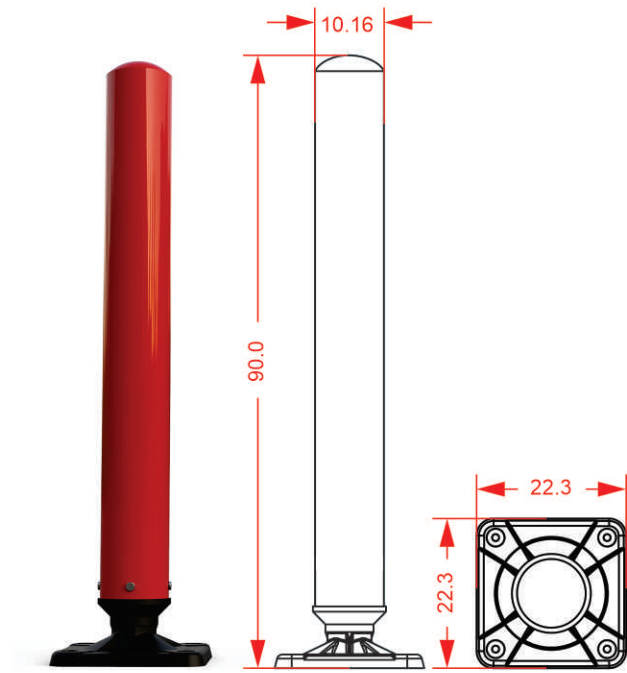
BOLARDO ABATIBLE
